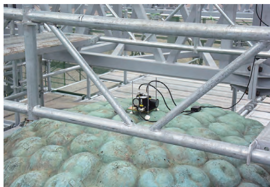
鎌倉大仏の常時微動測定調査 Microtremor measurement of the Great Buddha of Kamakura
